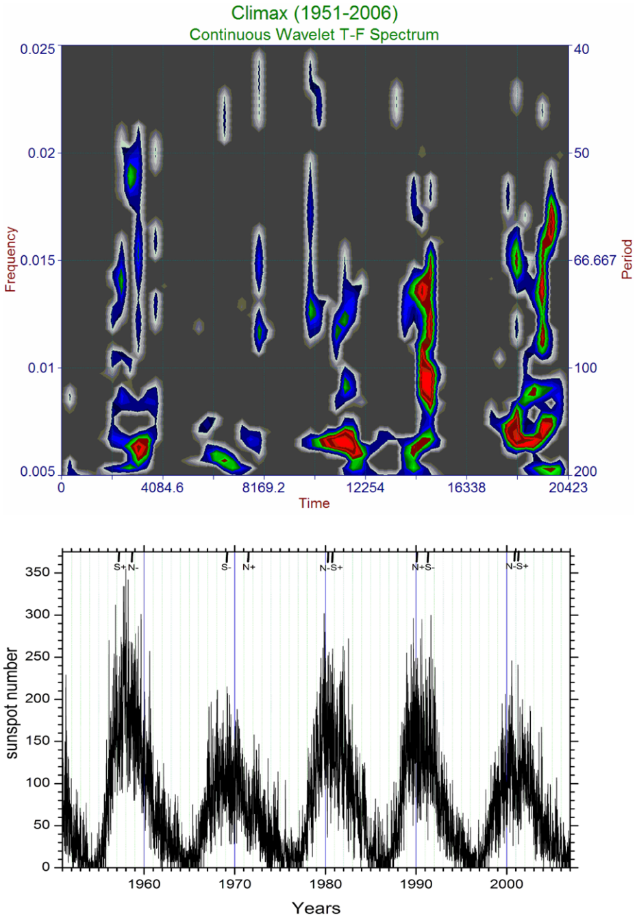
Figure 5 Upper panel: The wavelet time-frequency spectrum of the Climax neutron monitor. The abscissa is in days from 1 January 1951. The colour codes used are grey from 10 to 50%, cyan from 50 to 90%, green from 90 to 95%, yellow from 95 to 99%, and red from 99 to 99.9%. The Morlet mother function with the wavenumber parameter (the number of oscillations within the wavelet itself) of 16 is used. Lower panel: The smoothed sunspot numbers from http://sidc.oma.be/sunspot-data/ . The reversals of solar magnetic fields are marked.
