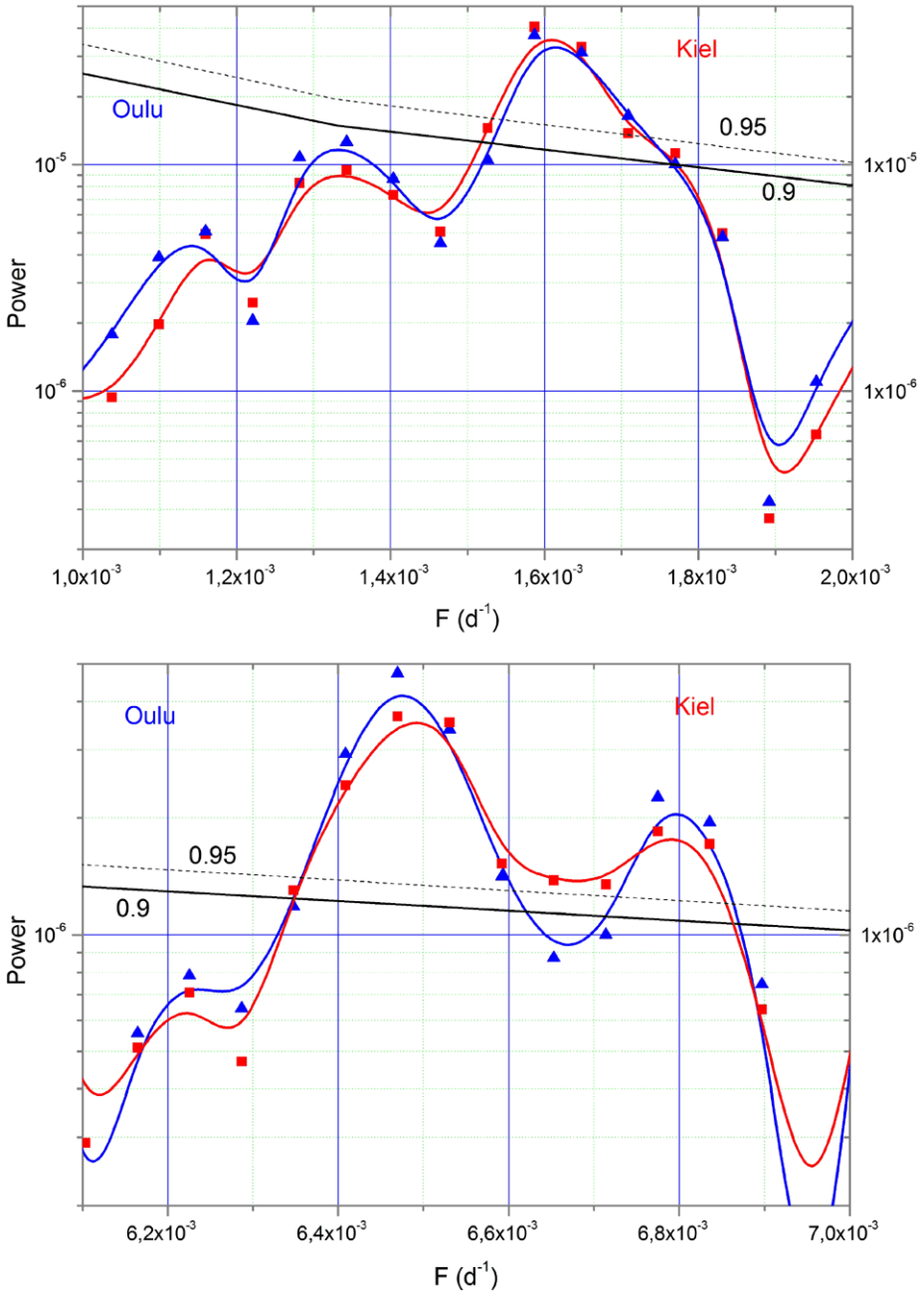
Figure 2 Power spectral densities (PSD) of neutron monitor time series at the two stations for the period shown in Figure 1. A B-spline technique is used for the curves plotted. The full line and dashed line are significance levels of 90 and 95%, respectively. The peak around 1.7 yr (upper plot) and a double structure near 150 days (lower plot) are seen.
