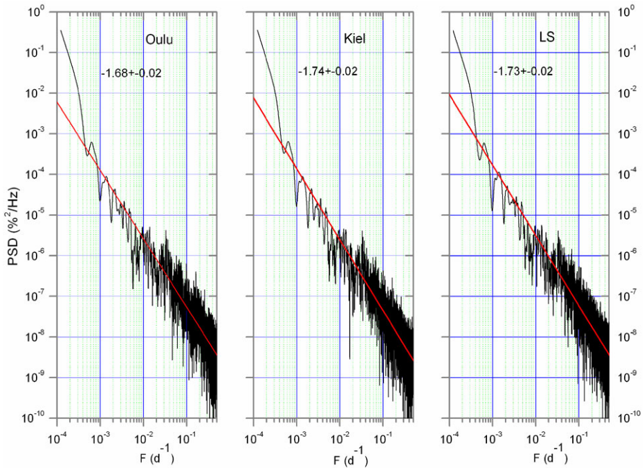
Figure 3 The power spectra of cosmic-ray time series measured at the three neutron monitors for the period shown in Figure 1. The data are normalised to 100% at the epoch of 1988.0794. The slopes of PSD are indicated with n according to the fit PSD(f) = \text{const.} \cdot f^{-n} .
