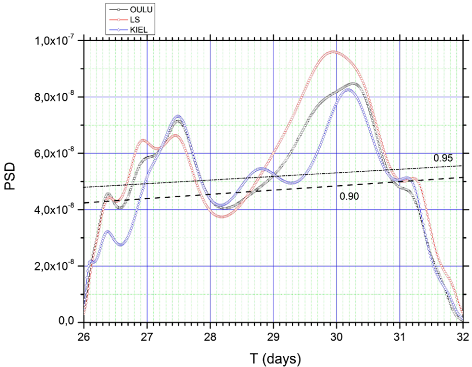
Figure 4 The periodogram (PSD as a function of period) around the solar rotation period at the three neutron monitor stations for the period shown in Figure 1. The dashed and dotted lines are significance levels of 90 and 95%, respectively.
