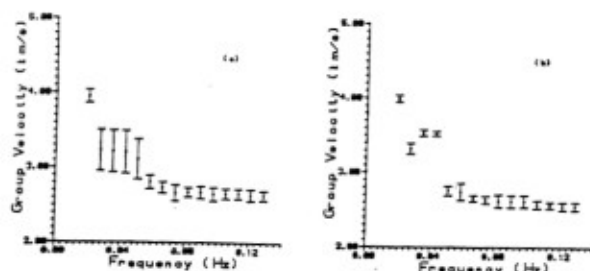
Fig. 2: Mean dispersion curves along the paths Chalkidiki-ATH (a) and Saros gulf-ATH (b) with corresponding 99.5% confidence intervals for each value of group velocity.
