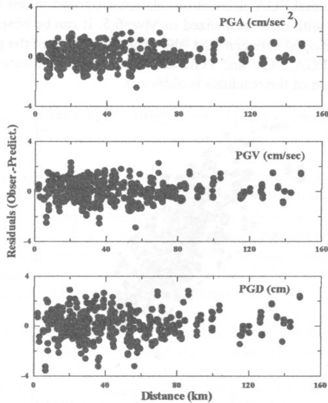
Figure 4: Distribution of the residuals of the peak ground acceleration, velocity and displacement in terms of distance.
