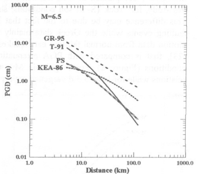
Figure 10: Comparison of the PGD empirical relations, Eqs. (7) (grey continuous line) and (8) (black dashed line), PS, with those proposed by Theodulidis [26], (black continuous line, T-91), Gregor [27], (grey dashed line, GR-95) and Kawashima [6] (black dashed line, KEA-86), for M=6.5 and rock soil conditions.
