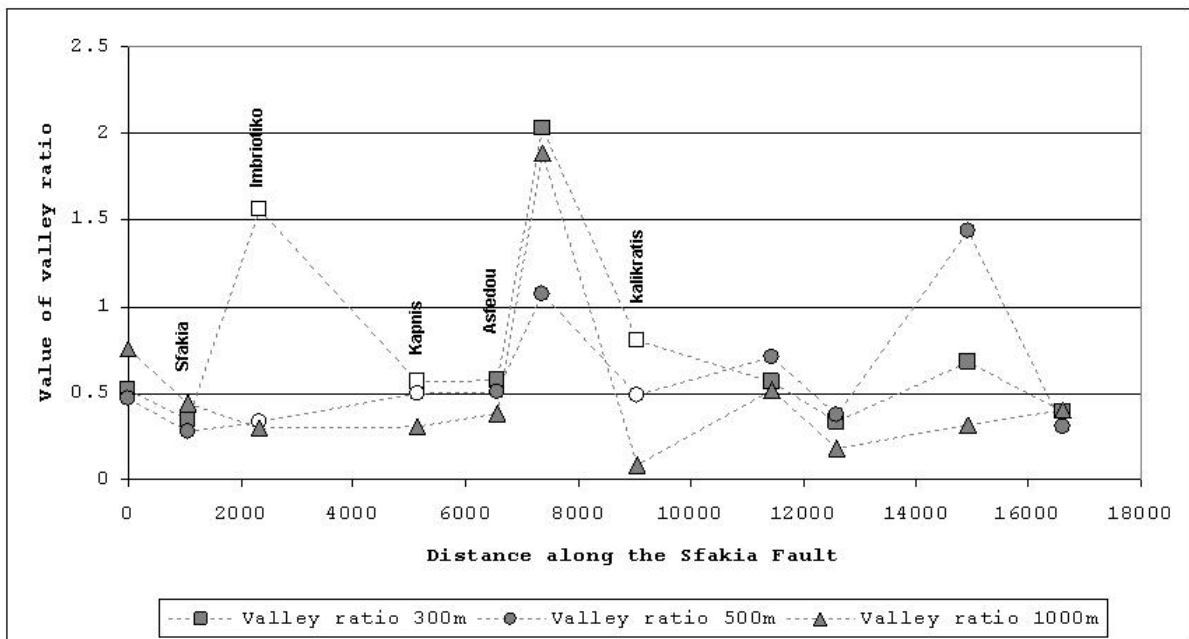
Figure 5: Graph showing the distribution of the ratio of valley floor width to valley height ( V_r ). The square points indicate values at 300 m distance from the Sfakia Fault while circles indicate values at 500 m distance and triangular points indicate 1000 m, respectively. The grey color means that the lithology of the valley is limestone. The white color means that the lithology of the valley is alluvial fan, scree or talus. The position of the Sfakia fault was determined by the break in morphological slope.
