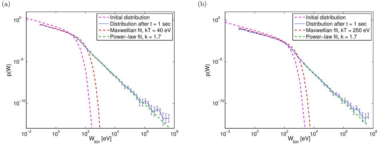
Figure 2. Energy distribution at t = 0 and t = 1 s of the electrons that have remained inside the box, for an initial temperature of (a) 10 eV and (b) 100 eV.
