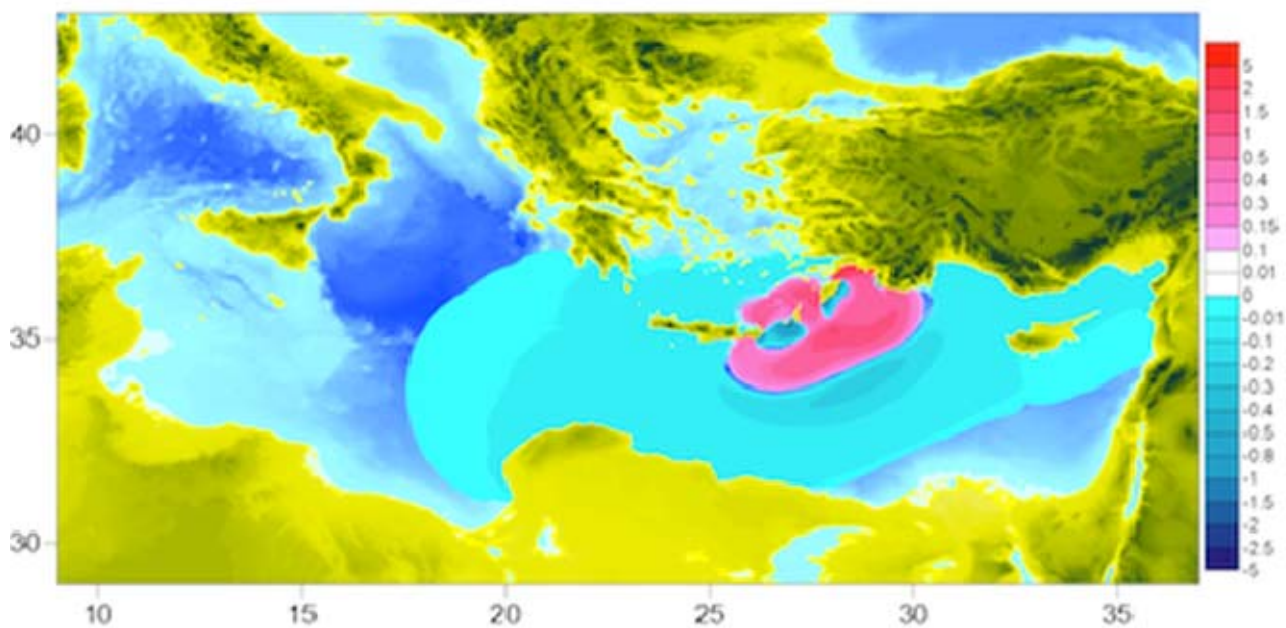
Figure 4 : Sea state after 10 mins for KOERI scenario.
