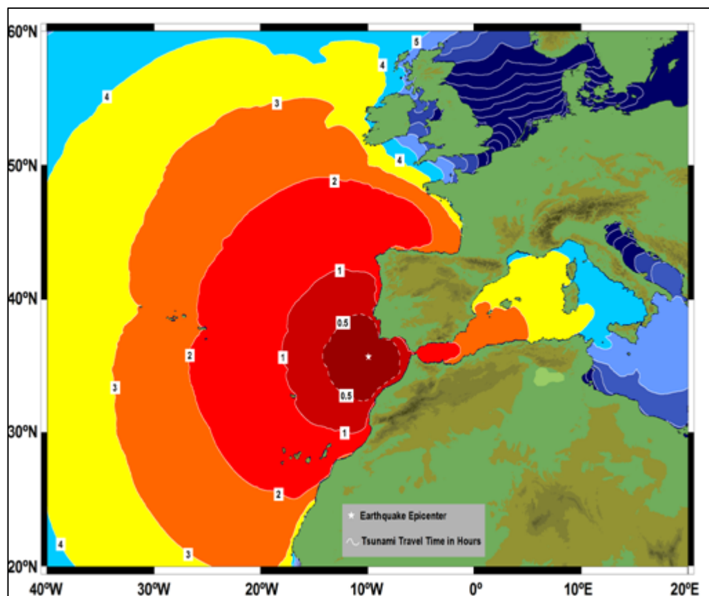
Figure 3 : Tsunami Travel Times. The point source corresponds to the epicenter of the proposed submarine earthquake.
