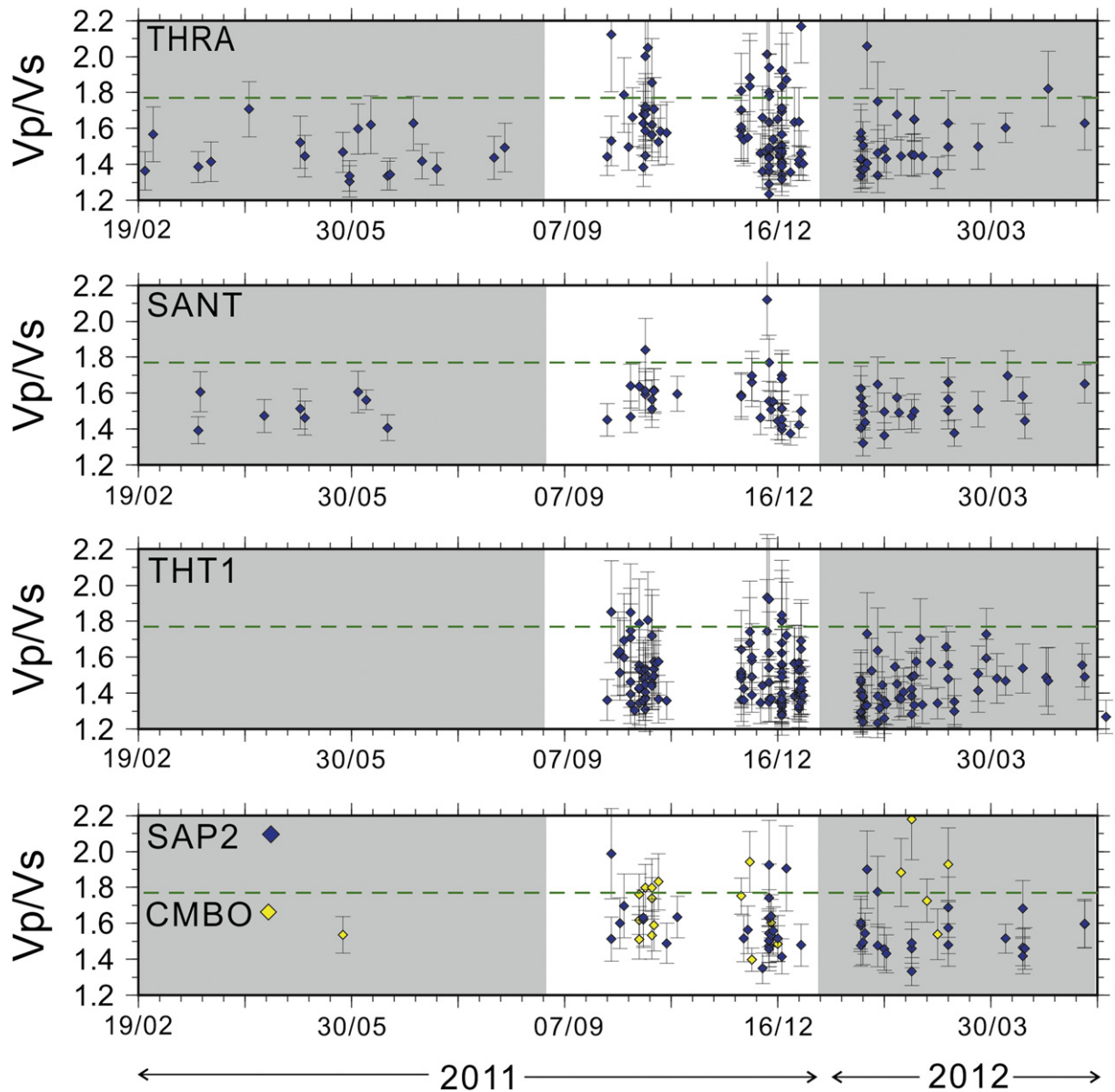
Fig. 7. Diagrams showing the variation of ray path averaged V_p/V_s ratio as a function of time for five different stations. The green line indicates the background V_p/V_s ratio ( \sim 1.77 ) for the Santorini area estimated by Dimitriadis et al. (2009). Shaded areas in each diagram highlight the three different deformation phases observed (see text for more details). Black vertical bars represent errors in measurement.
