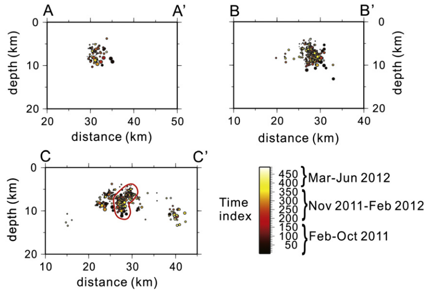
Fig. 6. Depth cross-sections showing the distribution of relative location hypocenters. The color scale given at the lower right hand side represents the index number of each event based on chronological order. The red curve delineates the two clusters that are located near the caldera rim between Nea Kameni and Thera islands.
