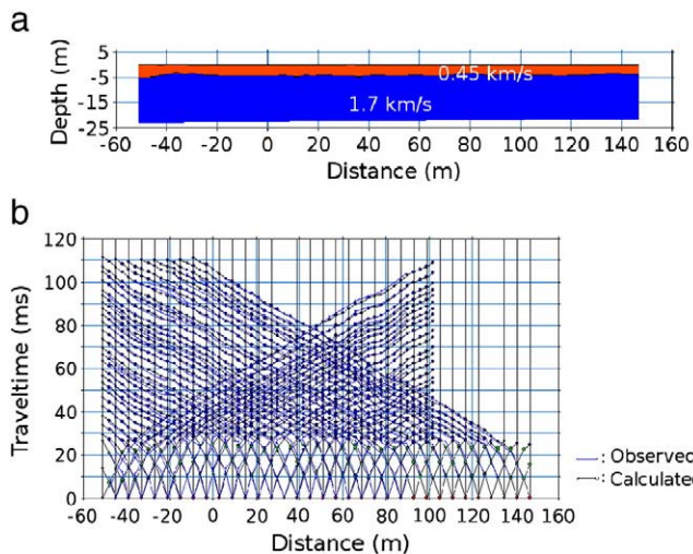
Fig. 18. An example of the water-table detection from a seismic refraction profile at the site WW'. (a) The resulted section. The velocity of the second layer is about 1.7 km/s. Since the S-wave velocity is about 0.15 km/s (see Fig. 17) the Poisson Ratio value approaches 0.5, i.e. the full saturation. (b) The fitting between the observed and calculated traveltimes was very good.
