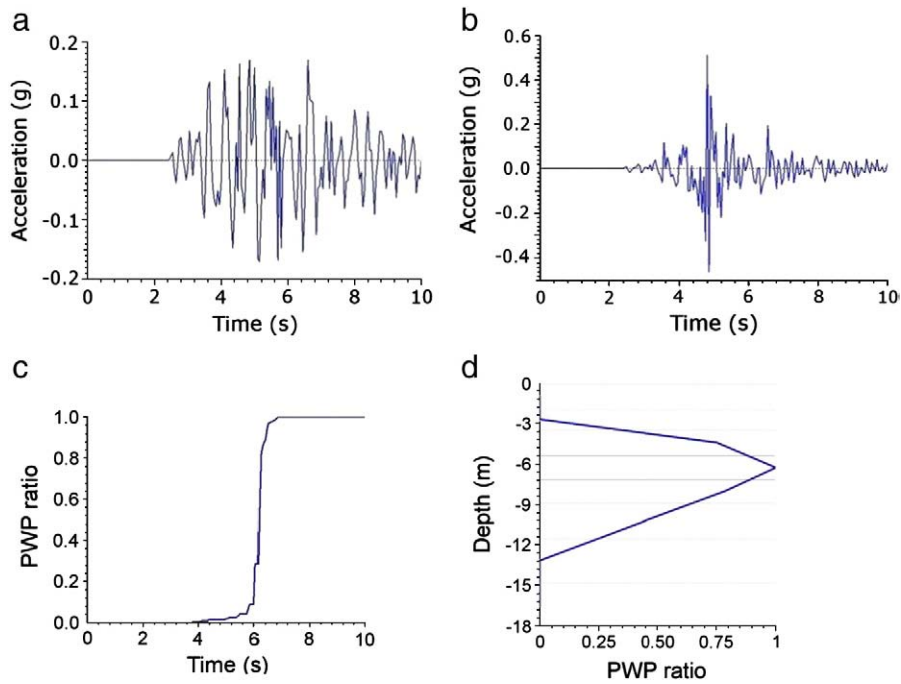
Fig. 19. Results of the liquefaction analysis for the AA' test site of Nafplion: (a) surface acceleration time history; (b) the acceleration time history at the potentially liquefiable layer; (c) the time history and (d) the depth distribution of pore water pressure ratio.
