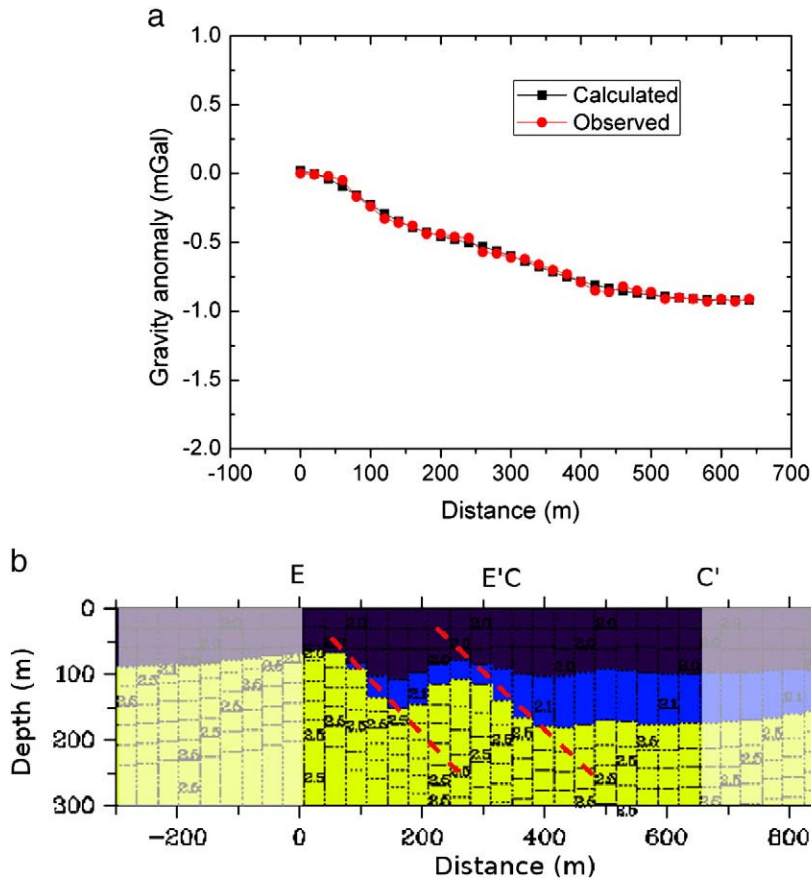
Fig. 13. (a) The fit between the calculated gravity data and the measurements was very good in the gravity profile EE'/CC'. (b) The resulted model.
