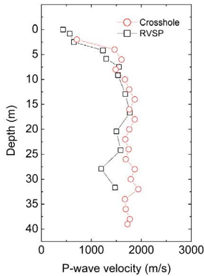
Fig. 15. Above: The velocity model of RVSP at the site KK'. Below: Comparison of RVSP with crosshole testing.
